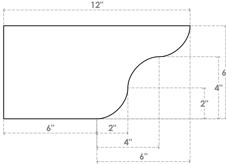
SIDE PROFILE
